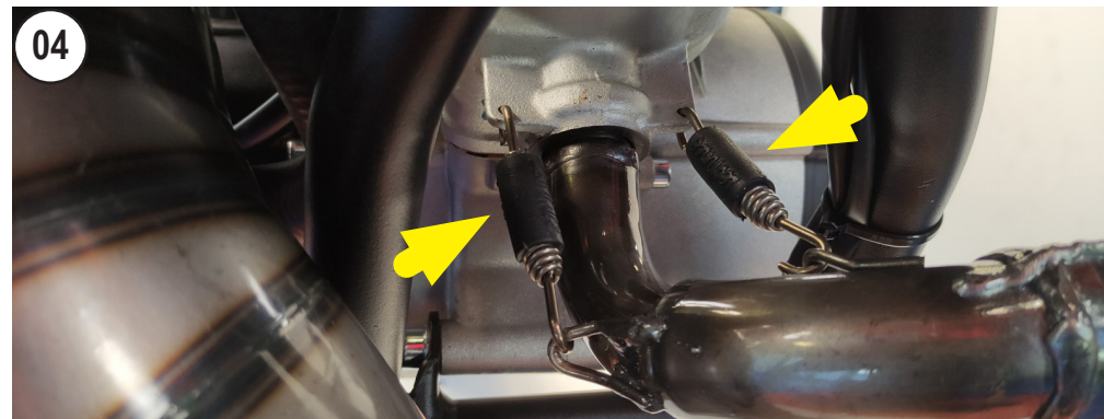
FIT THE LeoVince's HEADER PIPE AND HANG THE SPRINGS
