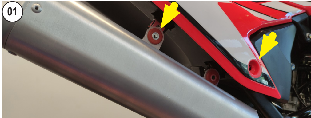
UNSCREW AND REMOVE THE STOCK MUFFLER
